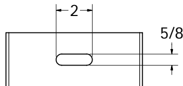
MOUNTING BRACKET DETAILS
